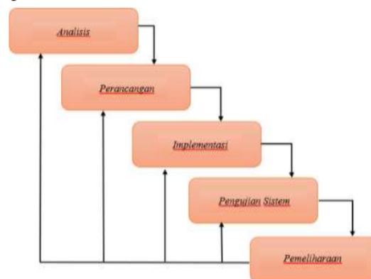
Gambar 2. Metode Waterfall
