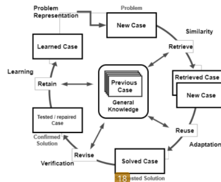
Gambar 1. Alur Kerja Case-Based Reasoning
