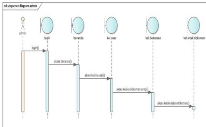
Gambar 5. Sequence Diagram admin
