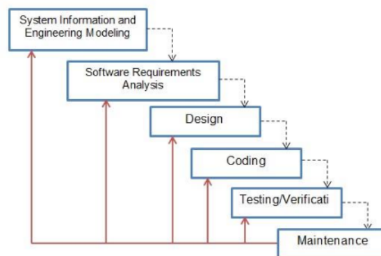
Gambar 1. Metode Waterfall
