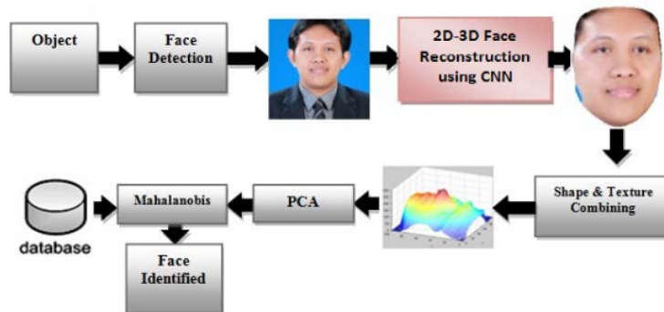
Fig. 2. 2D-3D image reconstruction process using CNN
