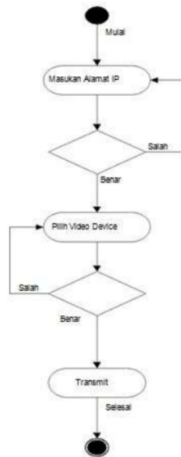
Gambar 5. Activity Diagram
