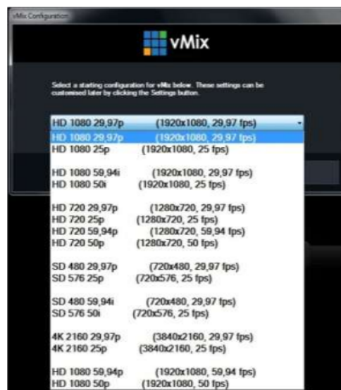
Gambar 10. Setting Resolution
