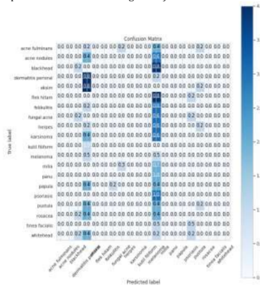
Gambar 7. Confusion Matrix
