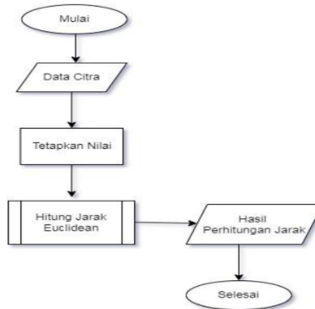
Gambar 5. Flowchart K-NN
