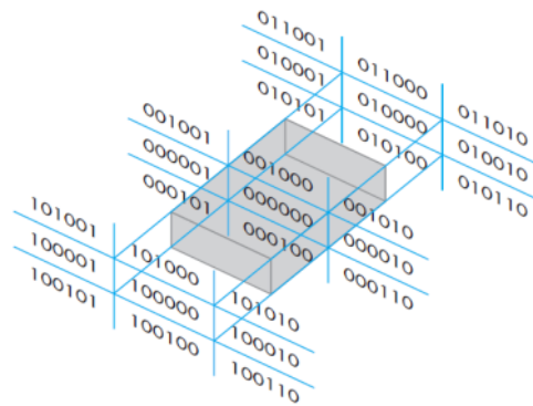
Gambar 9. Kode 6 bit algoritma Cohen-Sutherland (Angel dan Shreiner, 2012)
