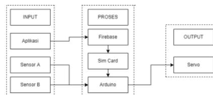
Gambar 1. Blok Diagram
