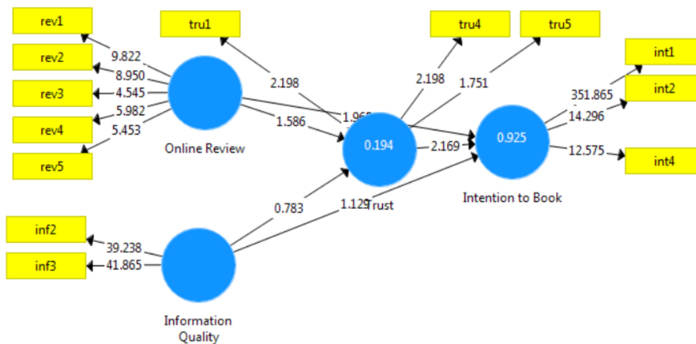
Gambar 1. Model Result
