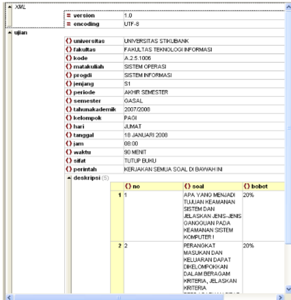
Gambar 2. XML Grid
