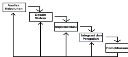
Gambar 1. Metode Waterfall
