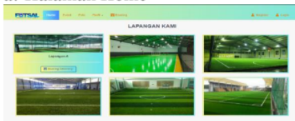
Gambar 4. Halaman Home
