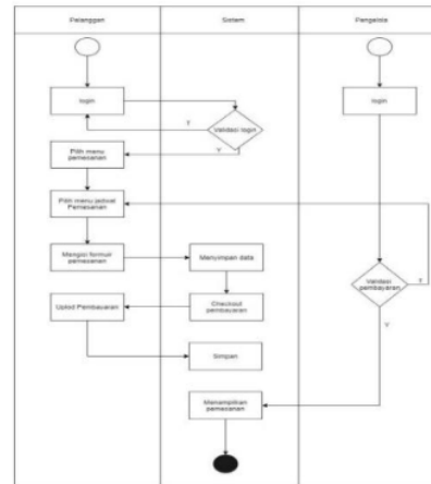
Gambar 3. Activity Diagram
