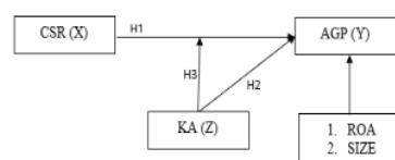
Gambar 1. Model Penelitian
