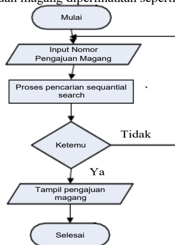
Gambar 1. Flowchart Pencarian Sequential Searching
