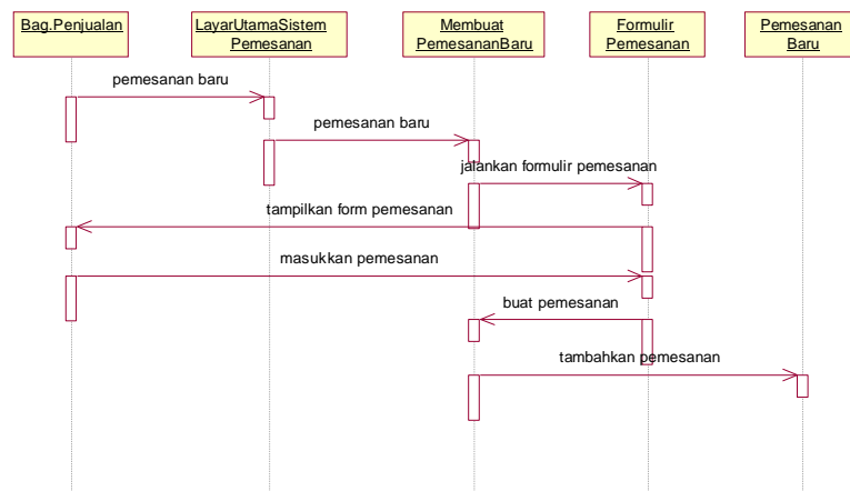
Gambar 3.19 Contoh Sequence Diagram
