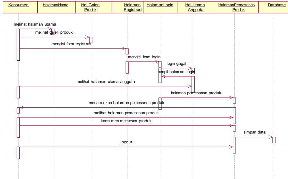
Gambar 4.4 Sequence Diagram User
