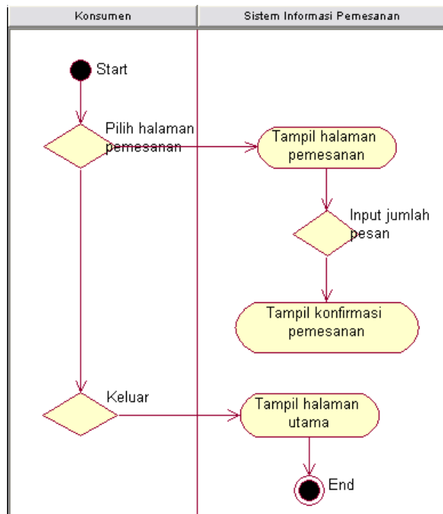
Gambar 3.21 Contoh Activity Diagram
