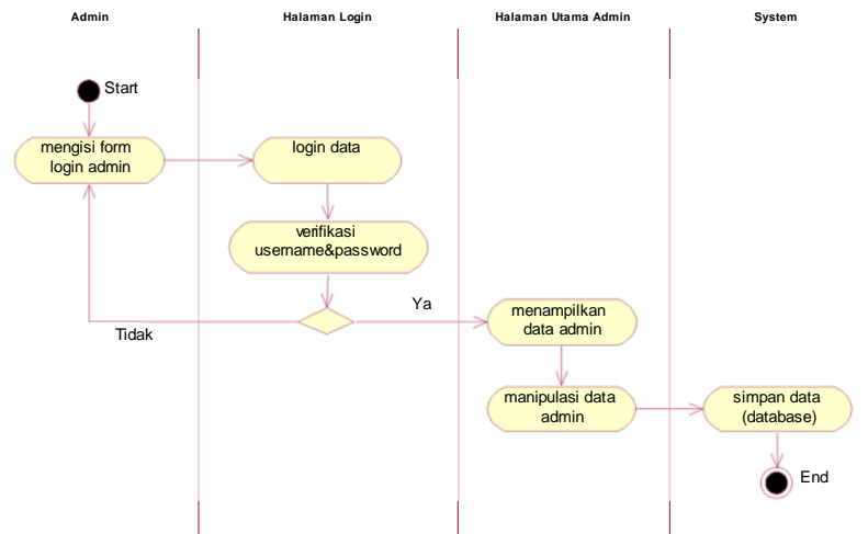
Gambar 4.3 Activity Diagram Admin
