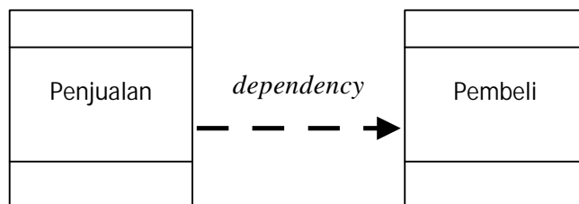
Gambar 3.12 Relasi Dependency
