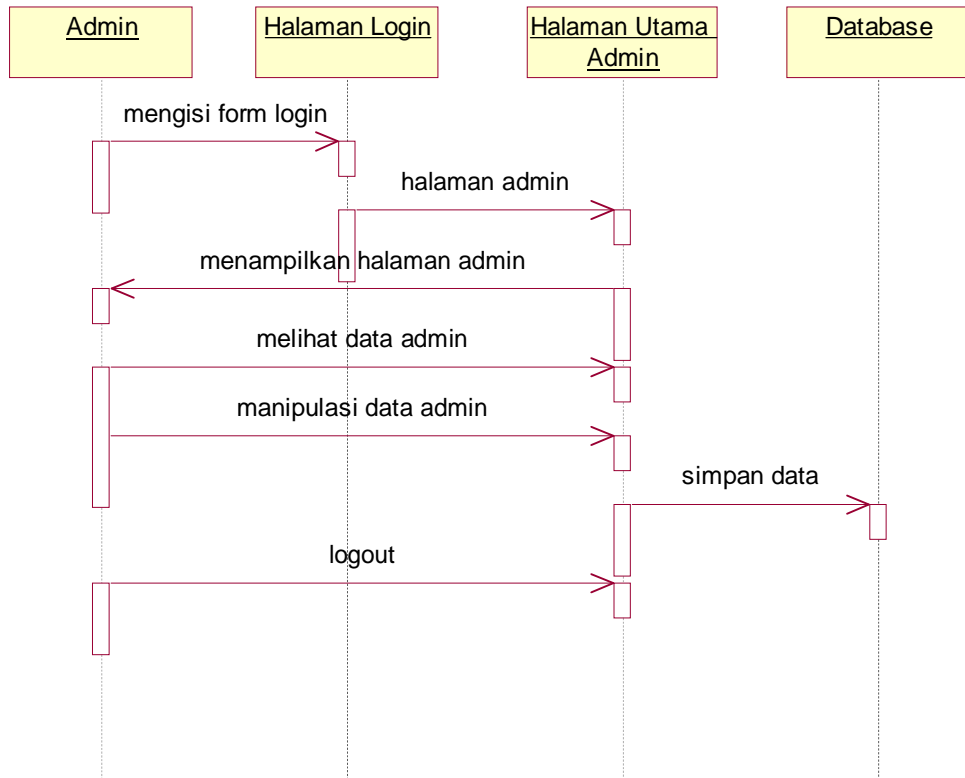
Gambar 4.5 Sequence Diagram Admin
