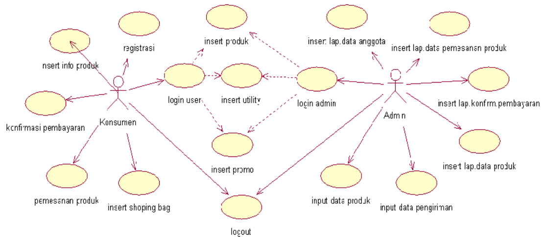
Gambar 4.1 Context Diagram
