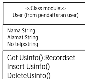
Gambar 3.9 Notasi Class
