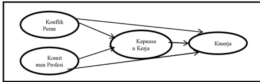
Gambar 1. Model Penelitian
