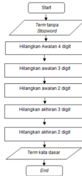
Gambar 10. Flowchart Proses Stemming
