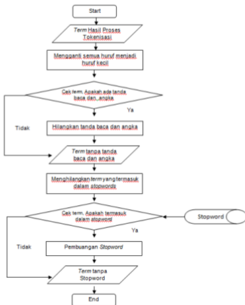
Gambar 9. Flowchart Proses Filtering
