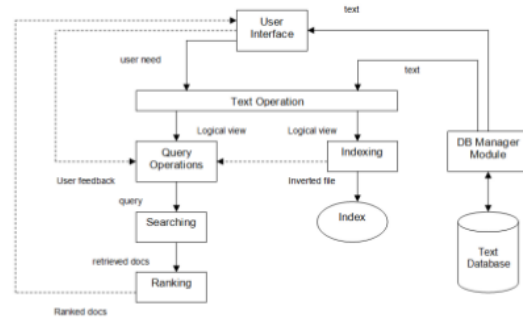
Gambar 1. The Process of Retrieving Information (Baeza, 1999.h.10)
