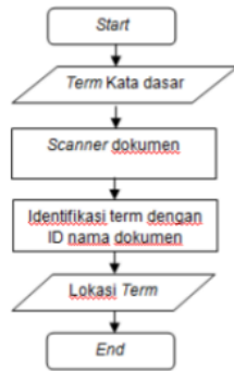
Gambar 11. Flowchart Proses Indexing
