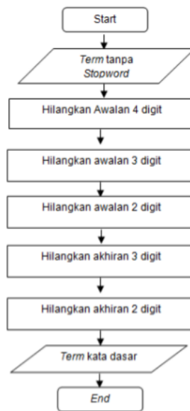
Gambar 3. Flowchart Proses Stemming
