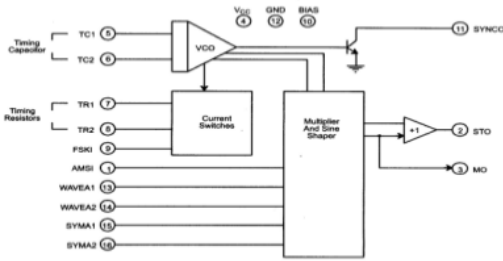
Gambar 1. Blok Diagram XR- 2206
