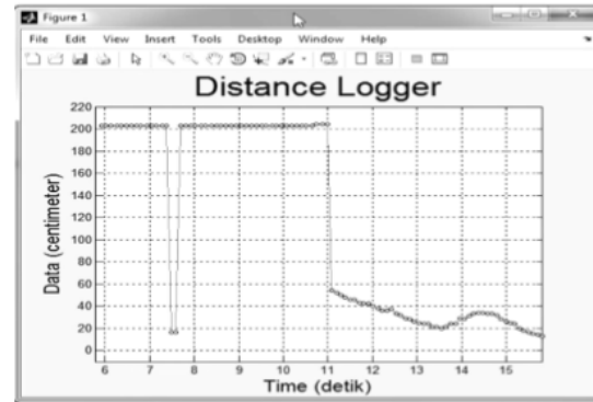
Gambar 4. Tampilan grafik plot distance logger .
