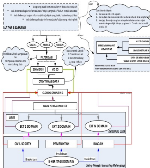
Figure 5. E-Heritage Data Processing System Architecture
