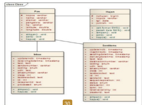
Gambar 7. Class Diagram
