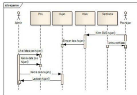
Gambar 8. Sequence Diagram
