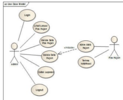
Gambar 6. Use Case Diagram
