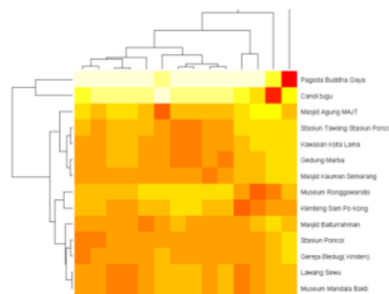
Gambar 5. Heatmap-Dendrogram
