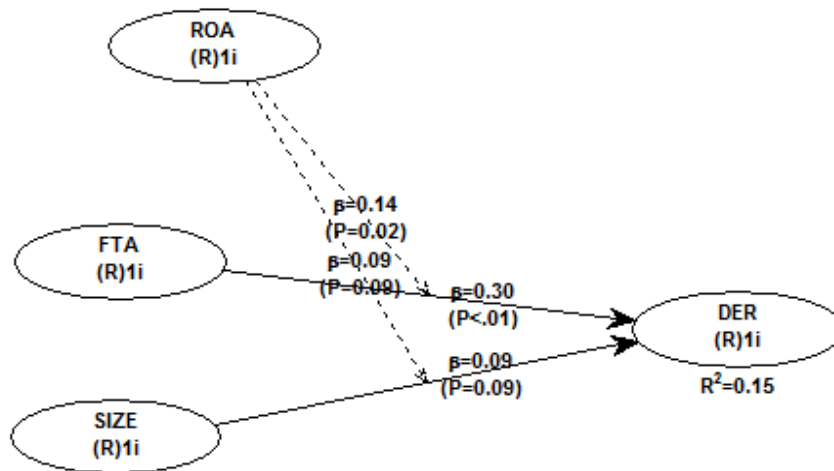
Figure 2. Findings of Structural Model
