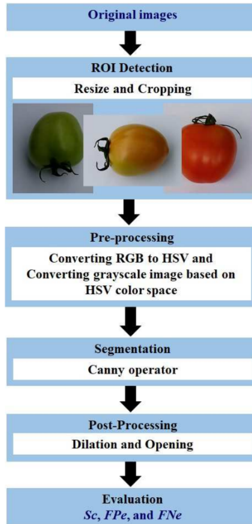
Fig. 2. The main processes of the tomato segmentation method
