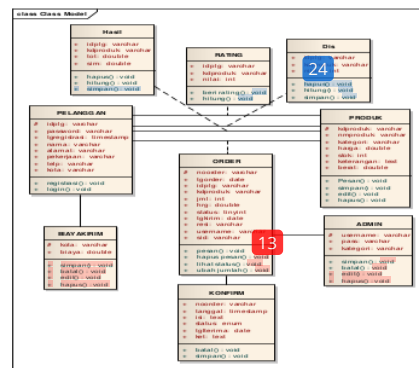
Gambar 3. Class Diagram
