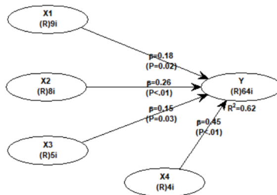
Gambar 1. Path Coefficients
