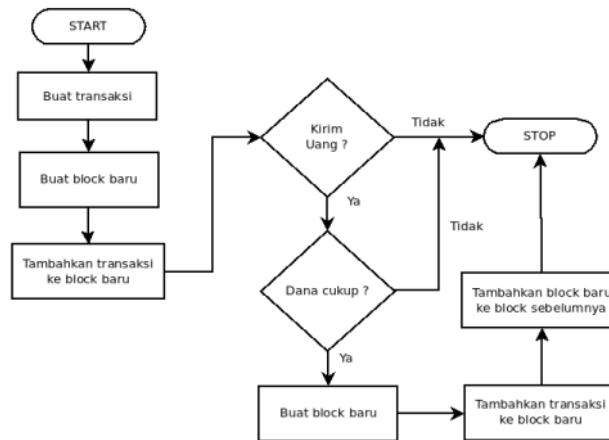
Gambar 2. Algoritma Blockchain.
