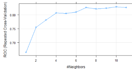
Gambar 4. Hasil perhitungan K-Nearest Neighbor berupa diagram
