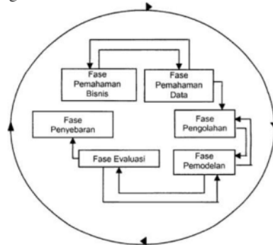
Gambar 1. Proses Data Mining menurut CRISP-DM
