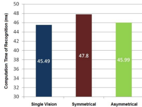
Figure 9. The Computation Time of Face Recognition (millisecond)
