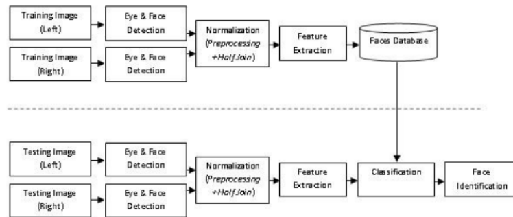
Figure 1. Face Recognition Using Asymmetrical Half-join Method
