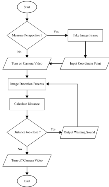
Figure 2. Flowchart work of application
