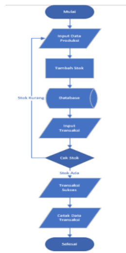
Gambar 1. Flowchart
