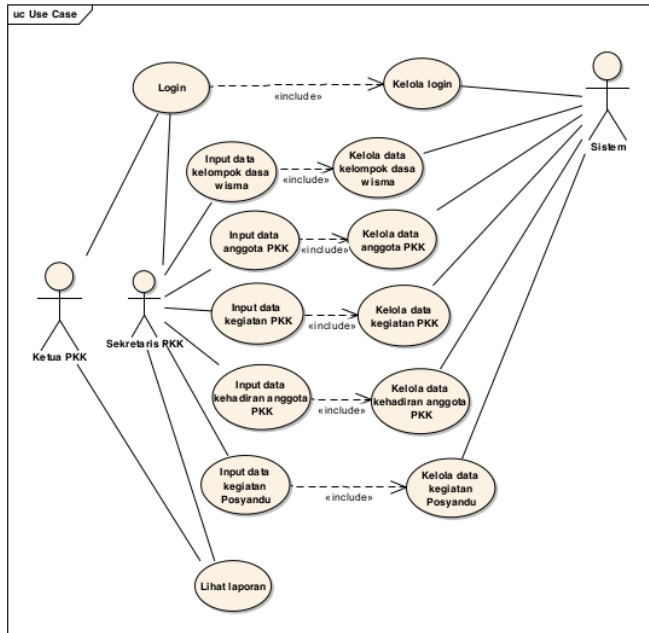
Gambar 2.1. Use Case Diagram
