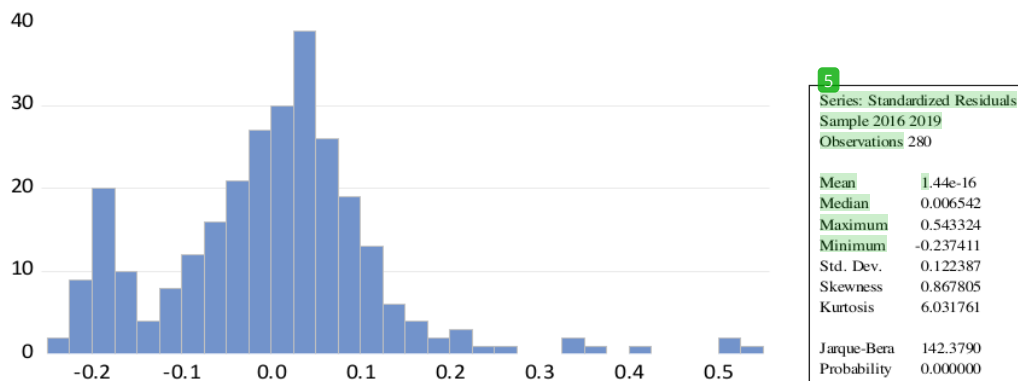
Figure 2. Normality Test
