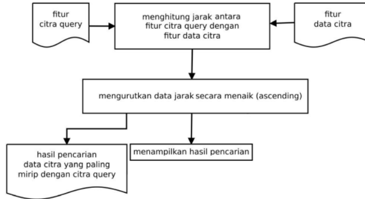
Gambar 1 Blok proses penelitian
