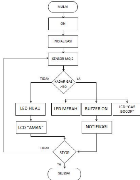
Gambar 3. Flowchart sistem
