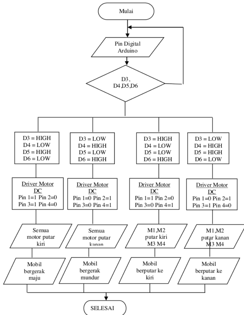
Gambar 4.2 Diagram Alir Sistem Kendali Robot Mobil
