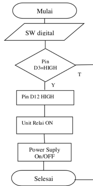
Gambar 6. Flow Chart Kendali Power Supply
