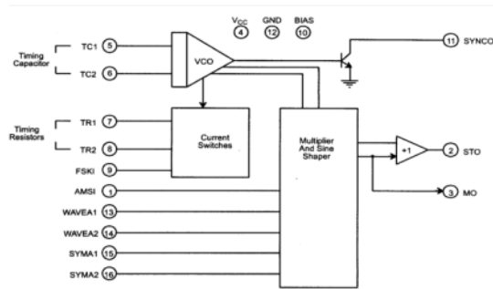
Gambar 2. Blok Diagram XR-2206
