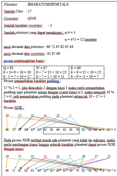
Gambar 4. Proses manual Pengujian Enkripsi PDAC
