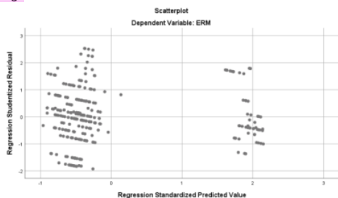
Gambar 3. Scatterplot
