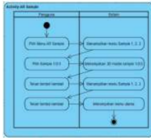
Gambar 4 Activity Diagram Ar Sample
