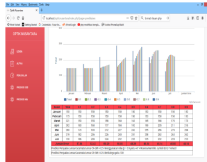
Gambar 2. Prediksi Single Exponential Smoothing
