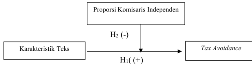
Gambar 1. Rerangka Penelitian
