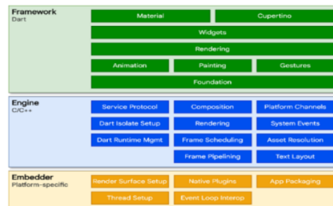
Figure 5. Flutter architecture
