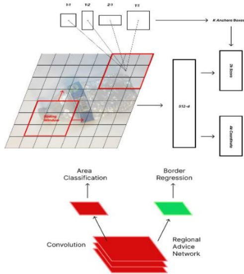
Figure 4. RPN architecture
