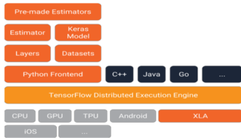
Figure 6. TensorFlow architecture
