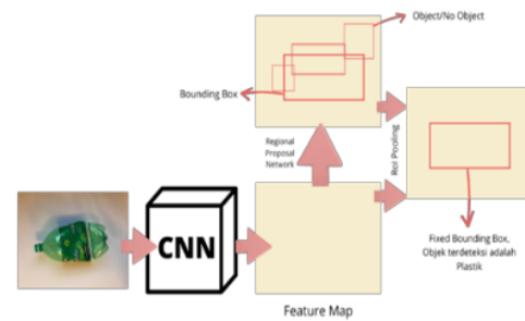
Figure 3. Faster R-CNN algorithm architecture
