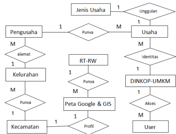
Gambar 2 Desain E-R Diagram
