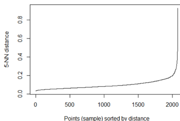
Figure 1. The KNN distance plot.
