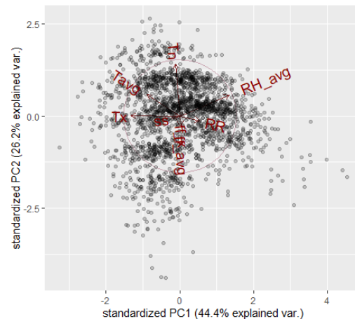
Figure 3. The PCA plot and the attributes axes.
