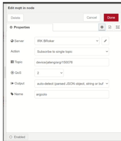
Fig 4. Configuration, Implementation of MQTT and Node-RED ARG
