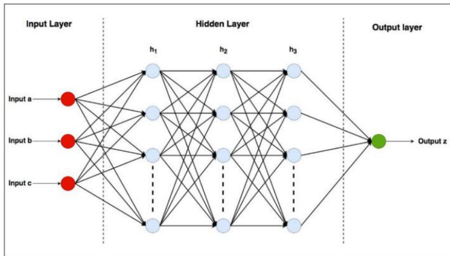
Gambar 1: Arsitektur Neural Network
