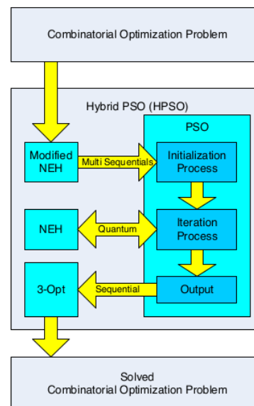
Figure 3 Combination model of NEH, PSO, 3-Opt algorithm
